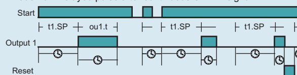
Mode 10 - Delayed pulse after continuous START signal
